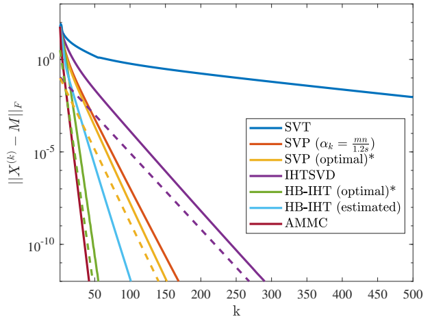
Fig. 1. The distance to the solution (in log-scale) as a function of the iteration number for various algorithms (solid) and their corresponding theoretical bounds up to a constant (dashed). Asterisks indicate algorithms using theoretical step sizes that are not available in practice. All algorithms share the same computational complexity per iteration except AMMC.
